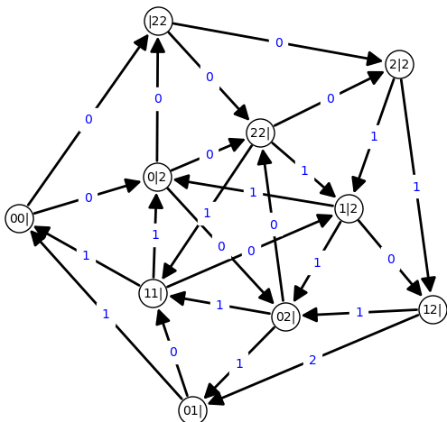
Figure 5: Graph of the category \mathcal{Y}_{2,2}
