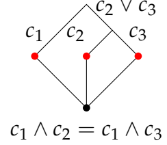
Figure 4: An antichain that is neither
