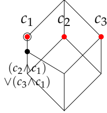
Figure 2: Strong not in- tersective
