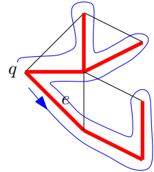
tree T and Bernardi tour
