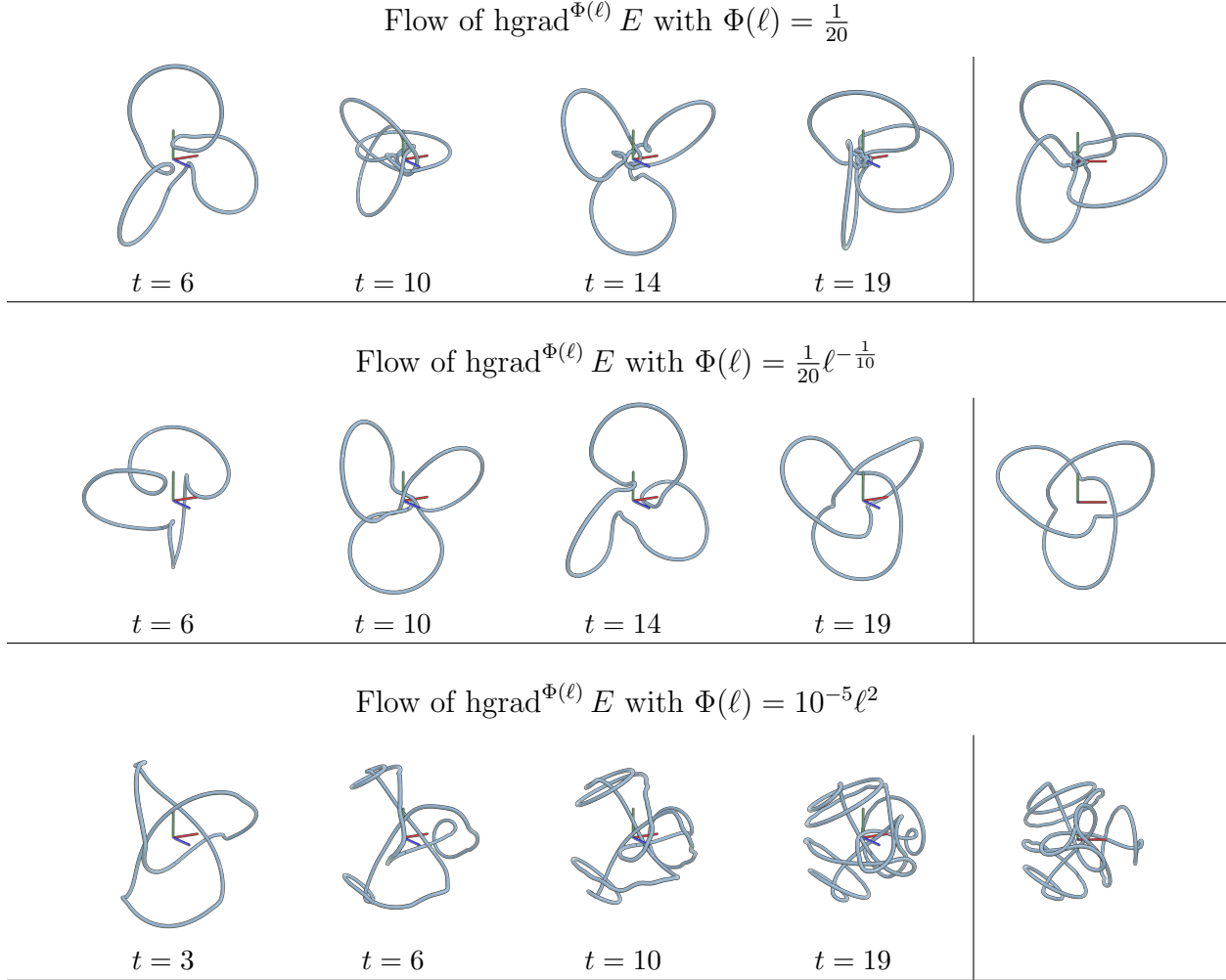
FIGURE 2. Hamiltonian flow of \text{hgrad}^{\Omega^{\Phi(\ell)}} E with different choices of \Phi(\ell) . In each row the initial curve, which is not shown, corresponds to the trefoil (11). The right-most images are the front-view of the last configurations of curves showing high symmetry for the 120-degree rotation around the z-axis.
